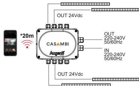
MatrixMini R 24Vdc - 16W HUB.24V.001.CA MAX 4 pz. 24vdc CASAMBI
